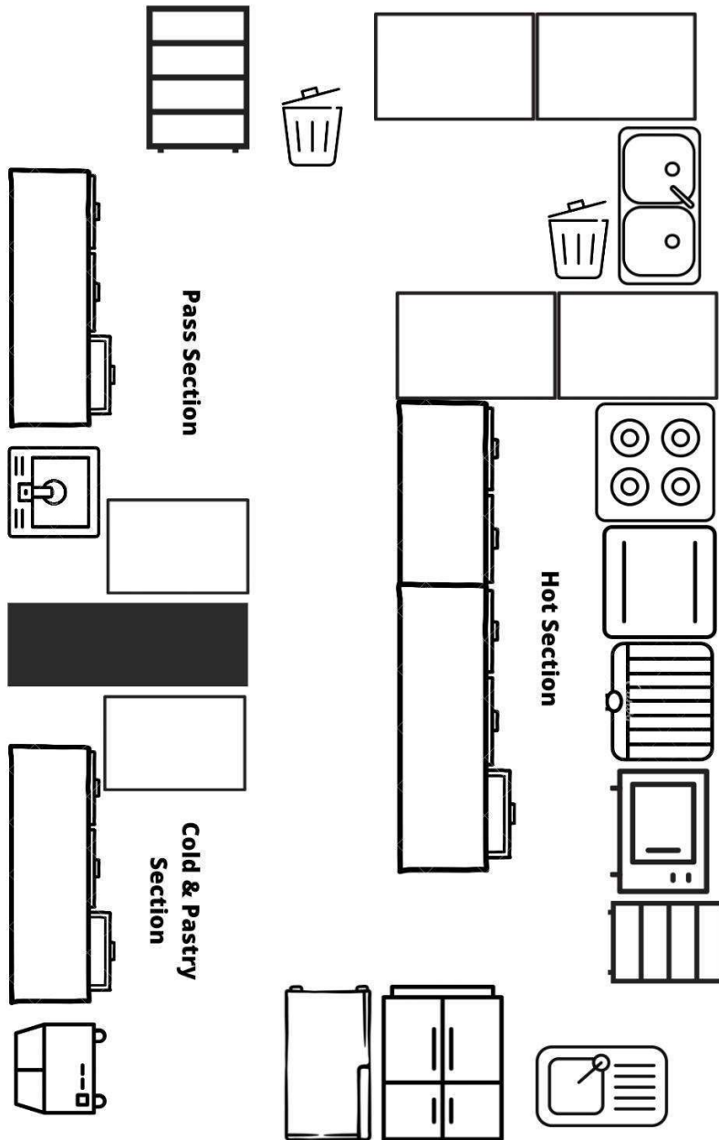
Figure 3.13 Kitchen Installation
